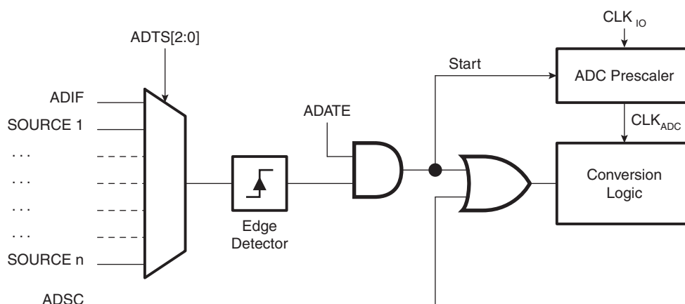
Figure 4-83. ADC Auto Trigger Logic
